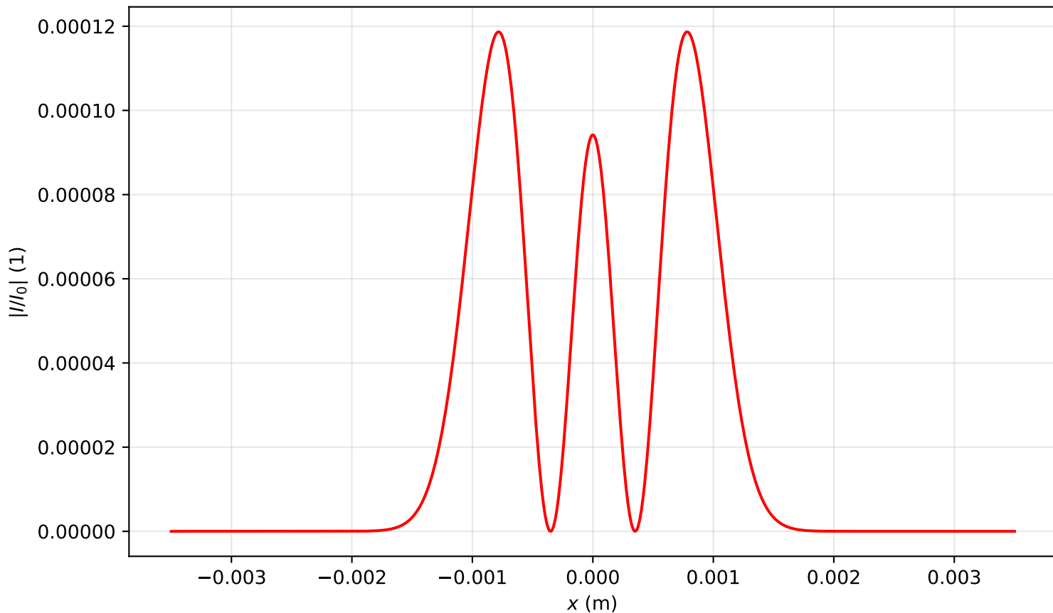
Intensity profile I(x, y = 0, z = 0.159)/I_0 , P_{in}=3.0P_{cr} , artificial time
